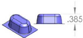
Medium Blister .385"
